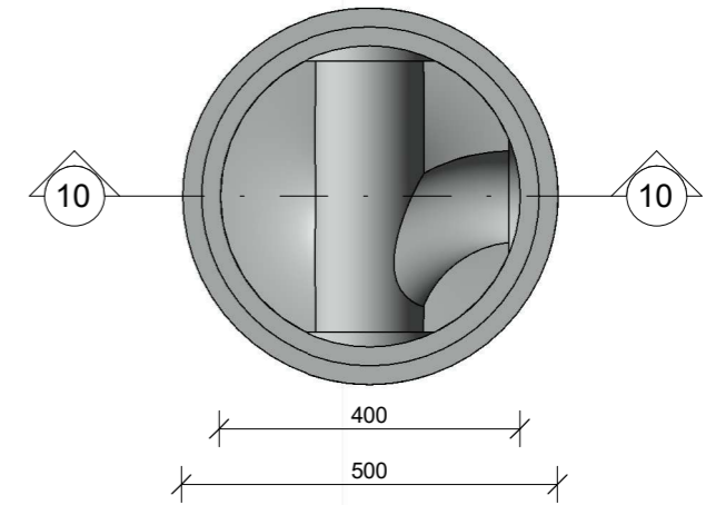
9 BASE A103 1:10
